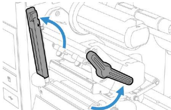
printhead and front arm lifted (PX940A)
